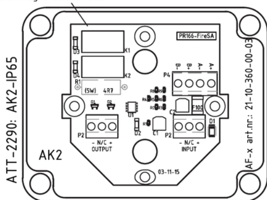
AF-X Monitoring & Control Unit
